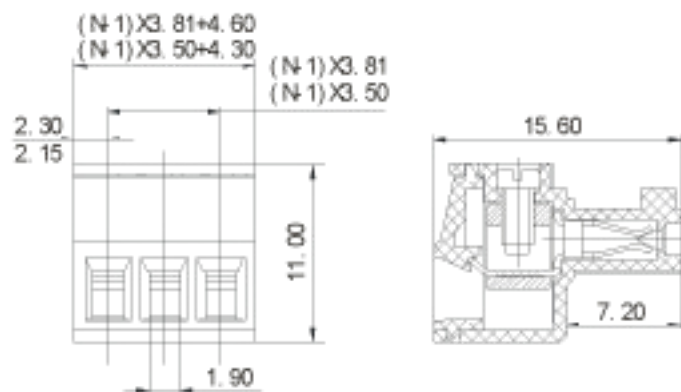
2EDGK-3.5/3.81
